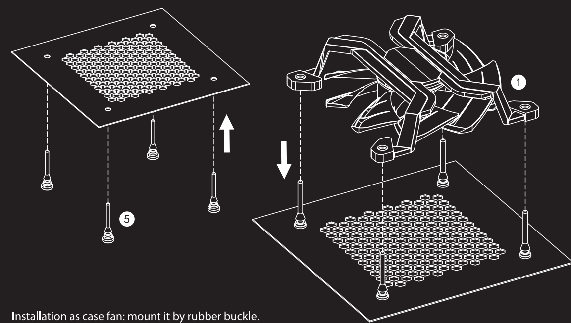
Installation as case fan: mount it by rubber buckle.
